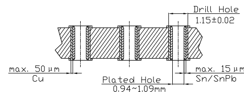
Recommended Hole Specifications Section A-A Scale 6:1
