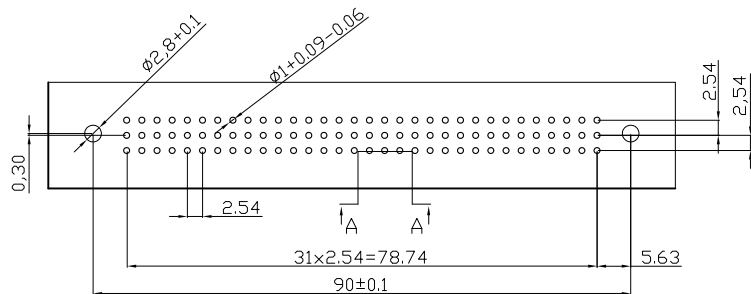
Recommended PCB Hole Layout Component Side Scale 1:1
